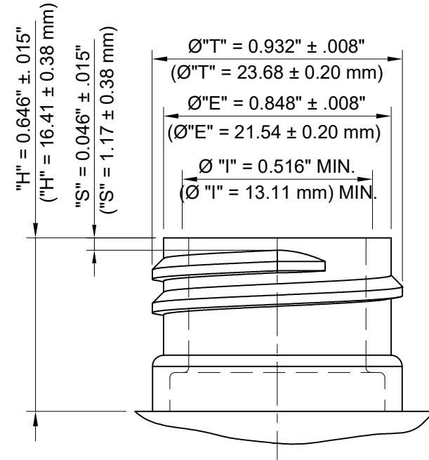
NECK DETAIL
