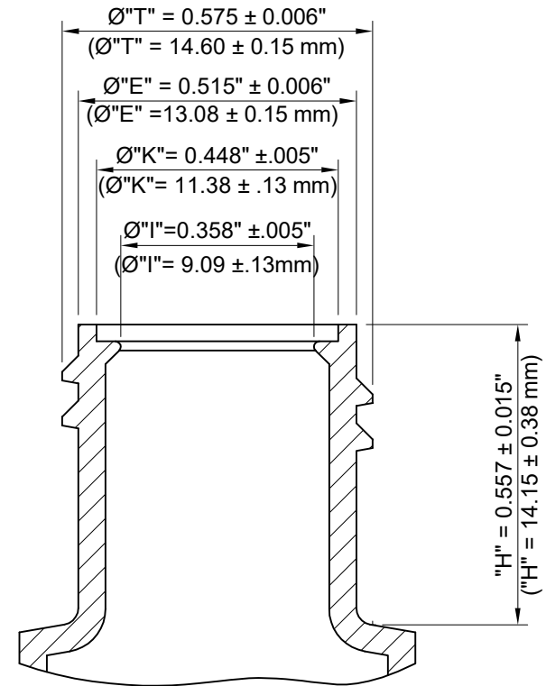
NECK DETAIL
