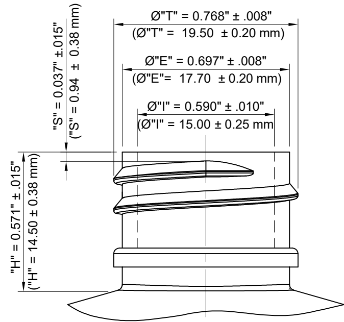
NECK DETAIL
