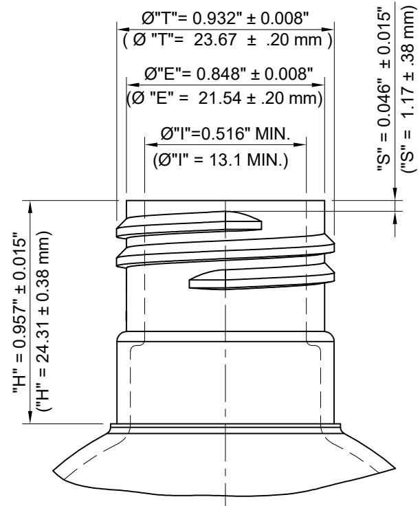
NECK DETAIL
