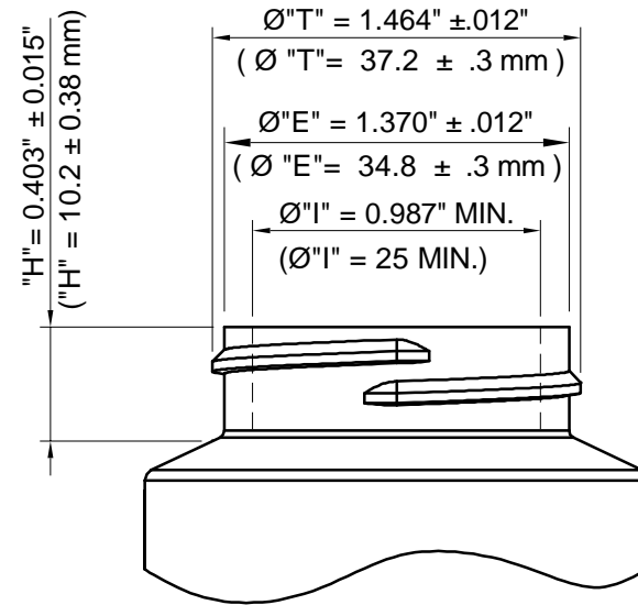
NECK DETAIL
