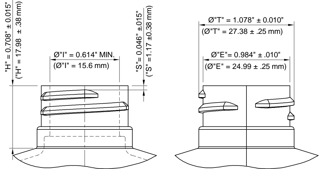
NECK DETAIL
