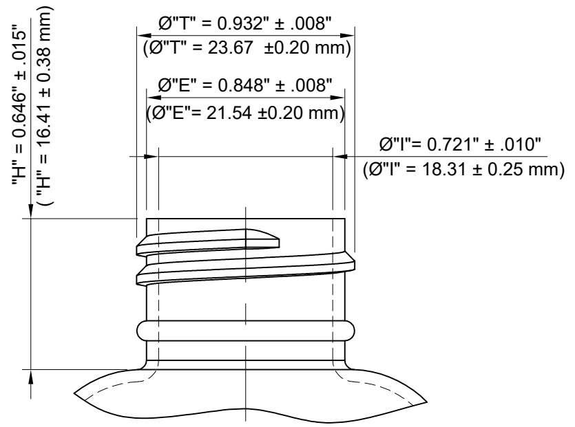
NECK DETAIL
