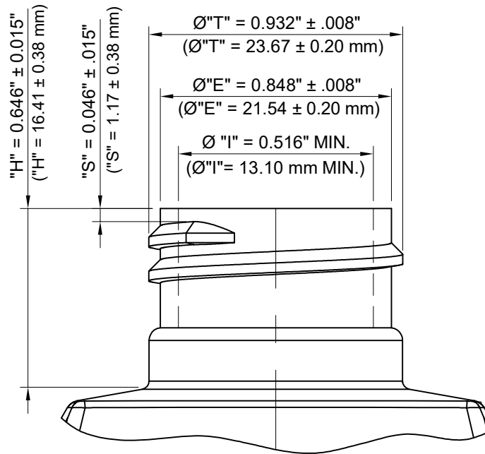
NECK DETAIL
