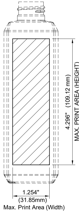
Right View
