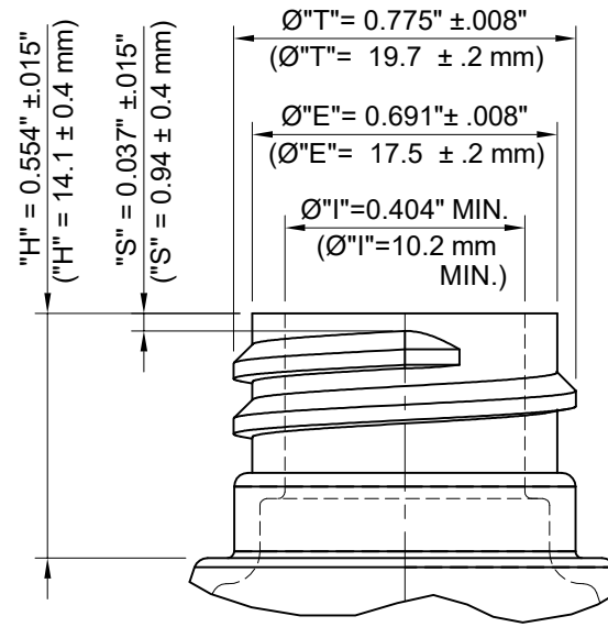
NECK DETAIL
