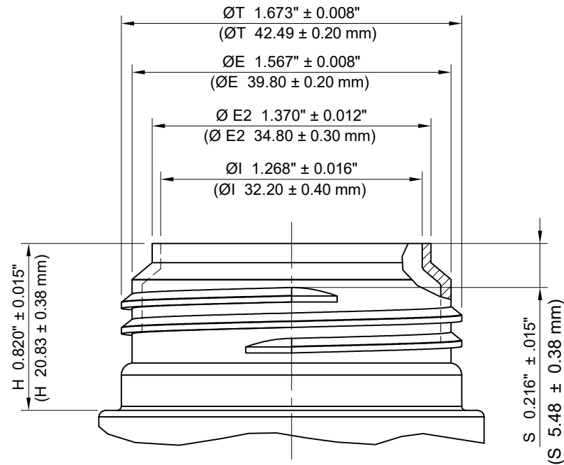
NECK DETAIL
