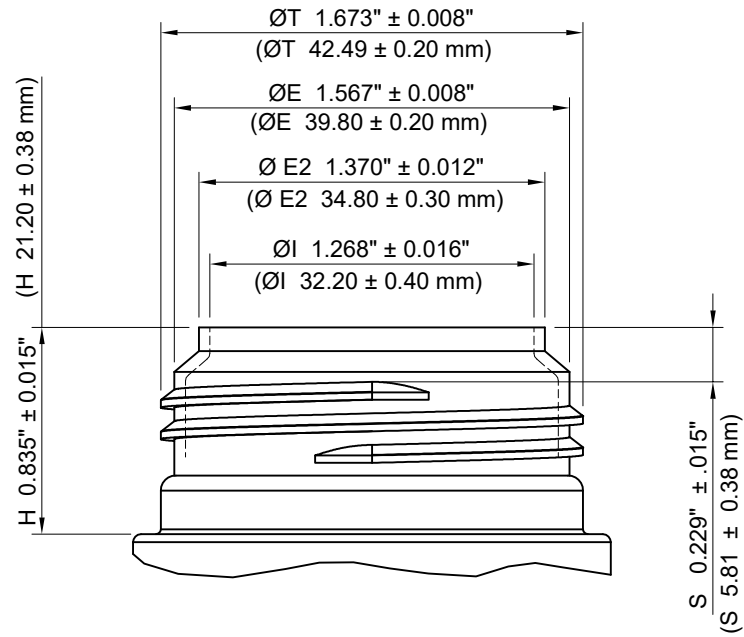
NECK DETAIL
