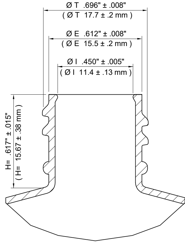
NECK DETAIL
