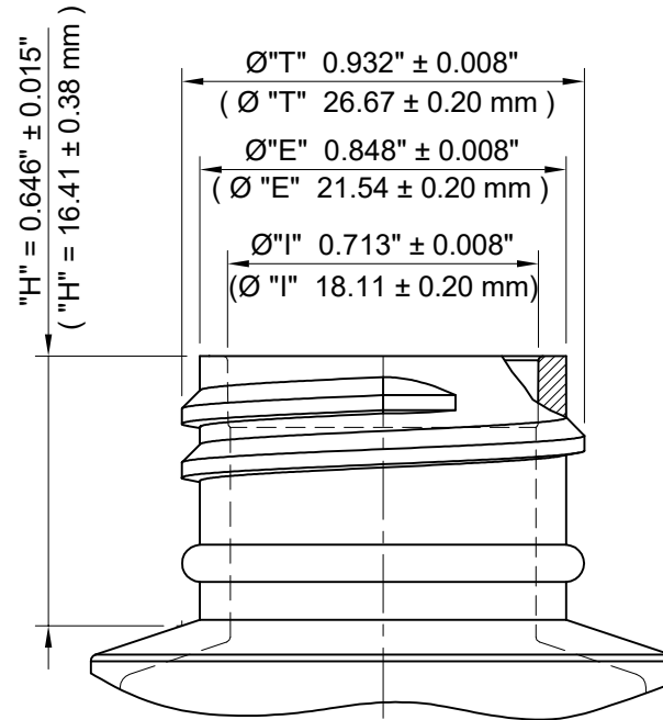
NECK DETAIL
