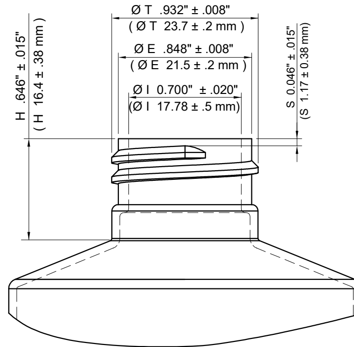
NECK DETAIL
