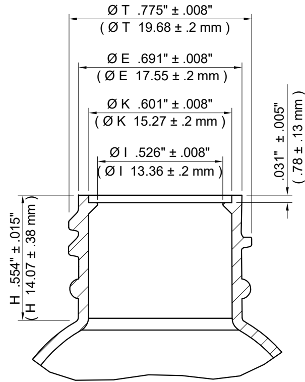
NECK DETAIL
