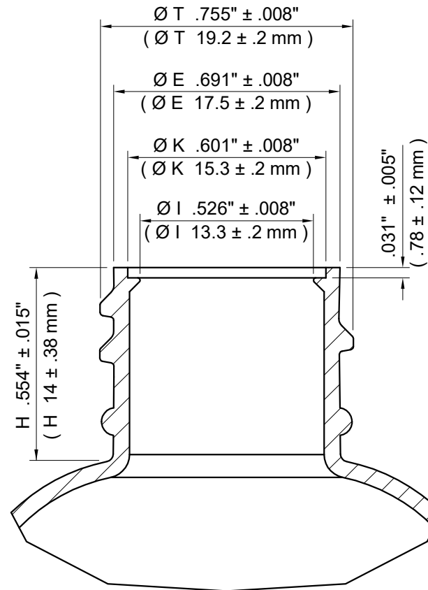
NECK DETAIL
