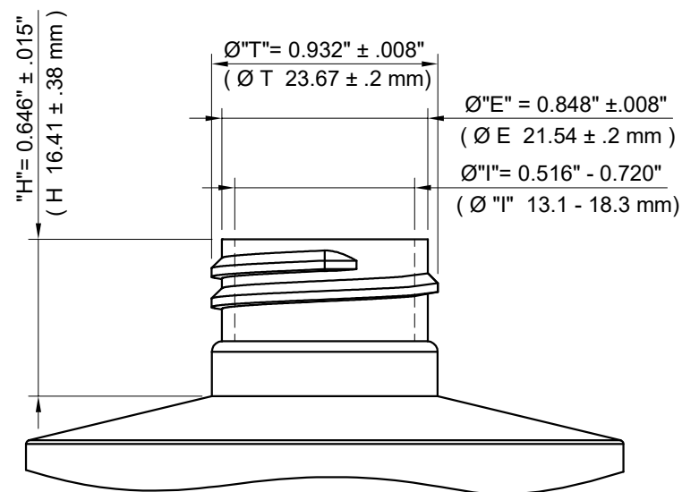
NECK DETAIL
