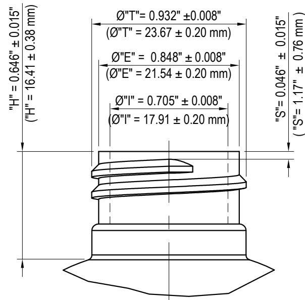
NECK DETAIL
