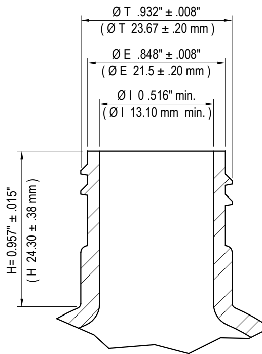
NECK DETAIL
