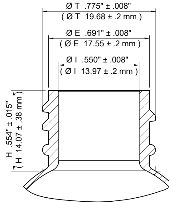
NECK DETAIL
