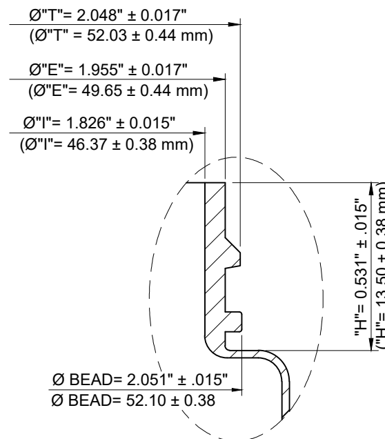
NECK DETAIL
