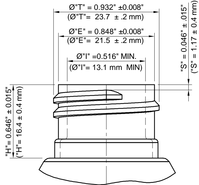
NECK DETAIL
