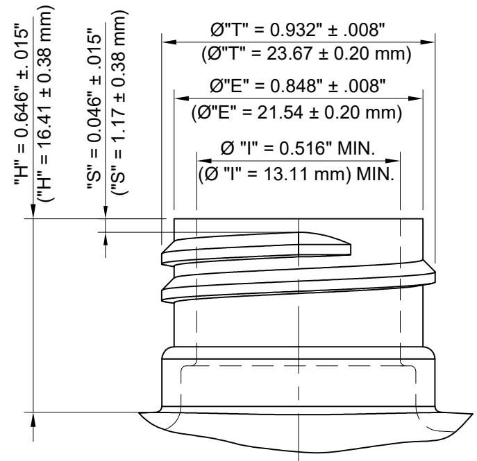
NECK DETAIL
