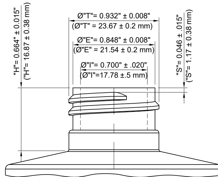
NECK DETAIL
