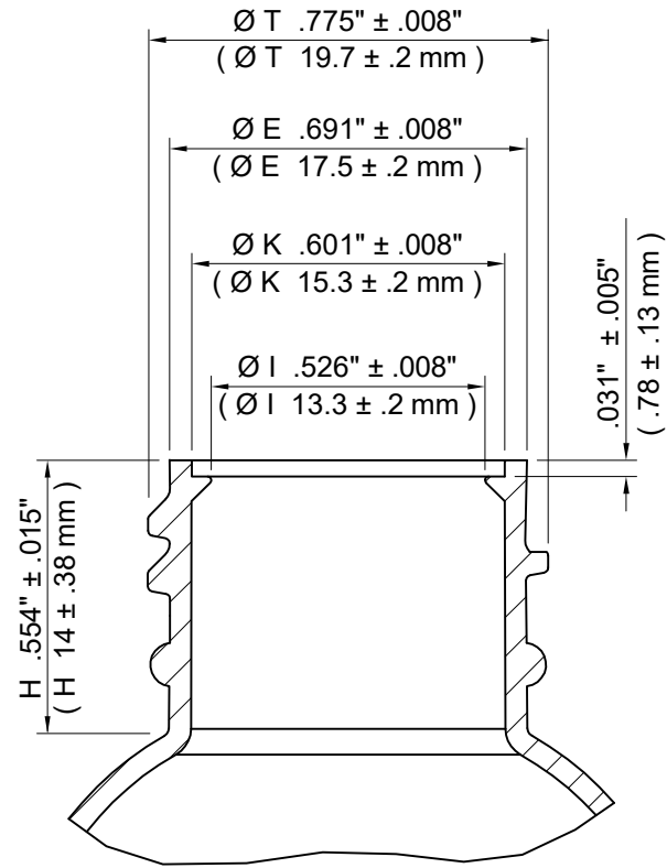
NECK DETAIL
