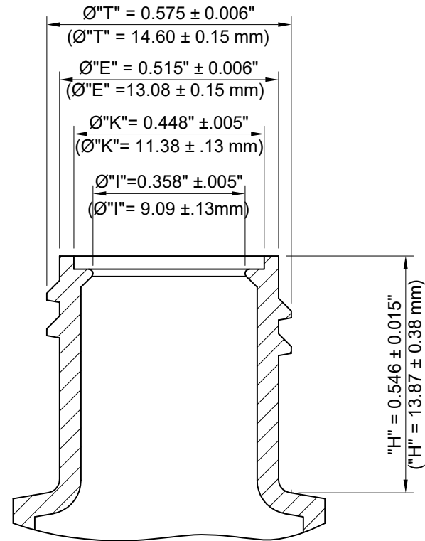
NECK DETAIL
