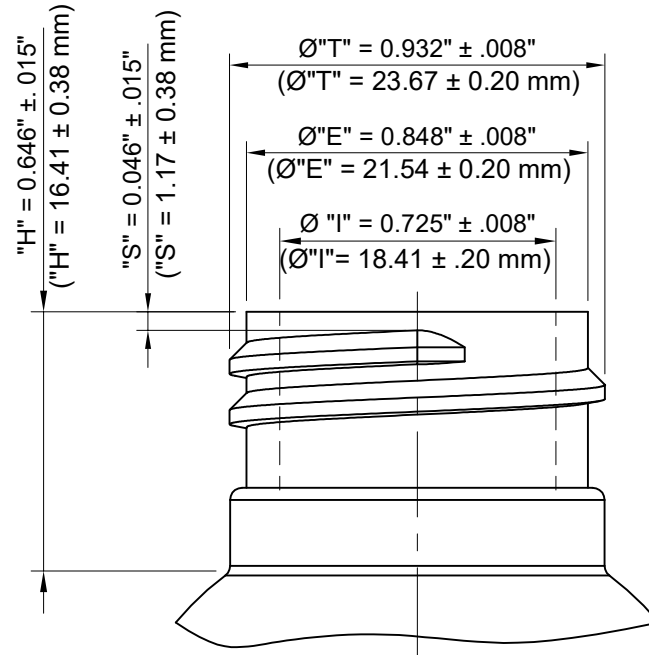
NECK DETAIL
