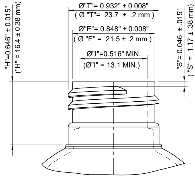
NECK DETAIL
