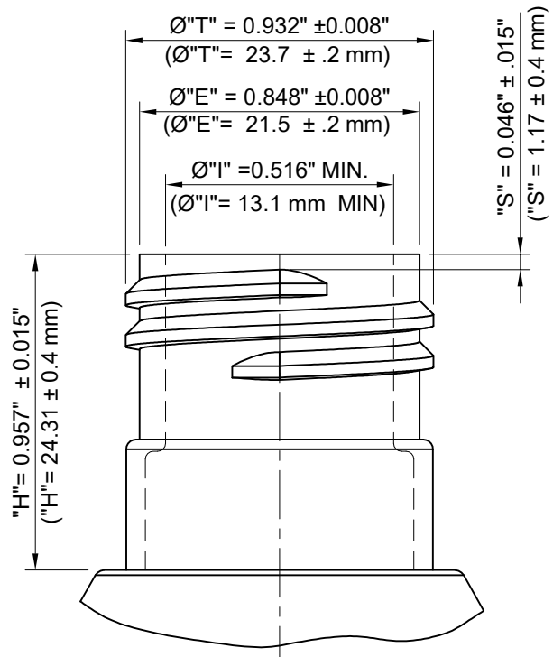
NECK DETAIL
