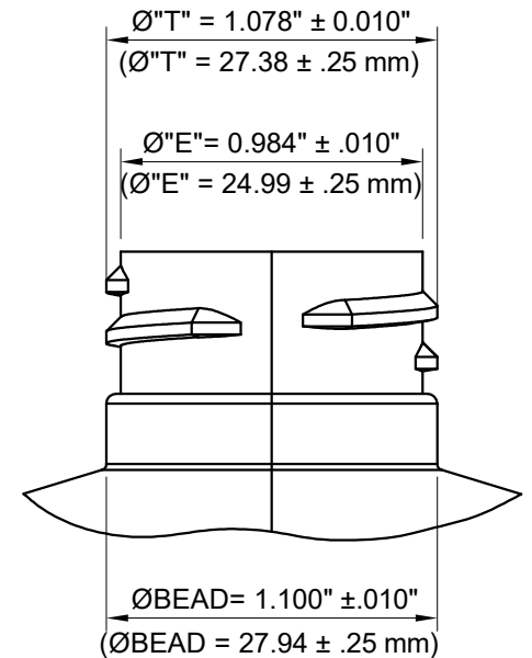
NECK DETAIL
